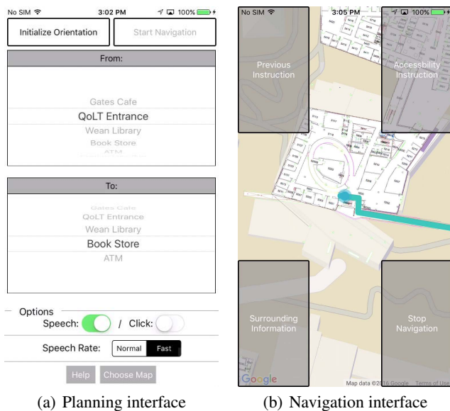
Figure 3. NavCog mobile interface
